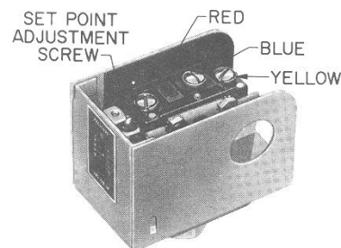
Fig. 2 -- Interior view of P10BG with terminals identified.
