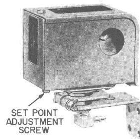
Fig. 1 -- The P10 Single Stage Pressure Control with barbed fitting and mounting bracket attached.
