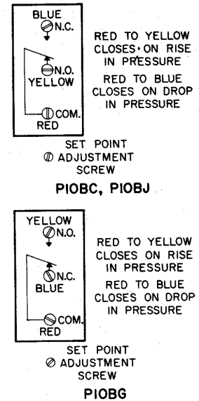
Fig. 7 — Terminal arrangement and cutout action.
